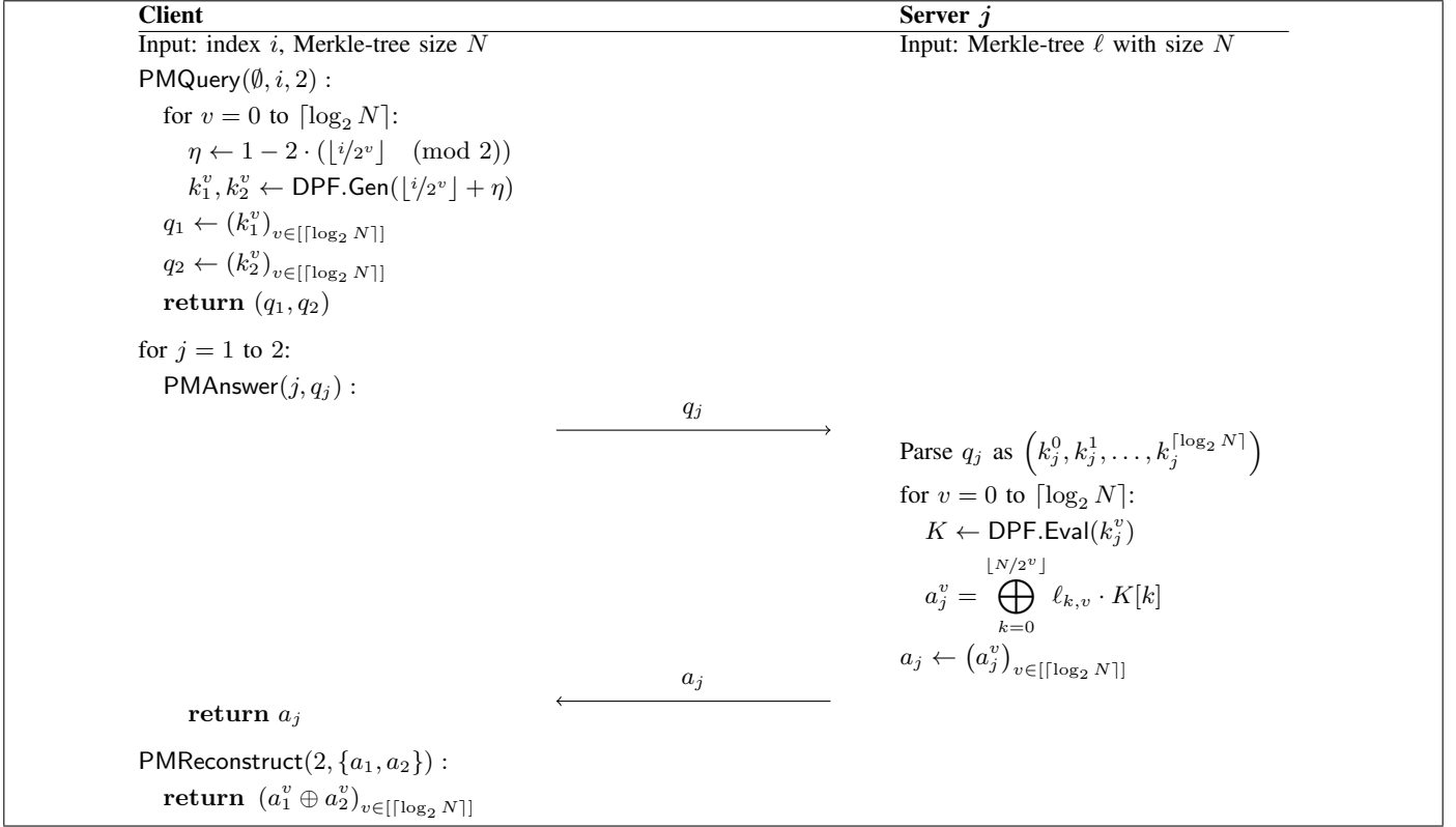
Scheme 6: Privacy-Preserving Retrieval of Membership Proofs instantiated with DPF-based PIR.
